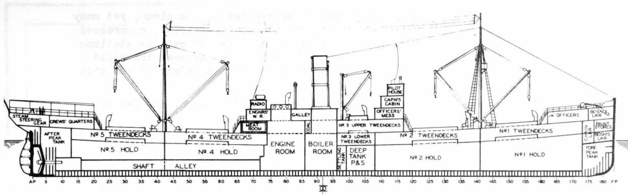
FIGURE 1 - S.S. PACIFIC EXPLORER (EX-MORMACREY) BEFORE CONVERSION
